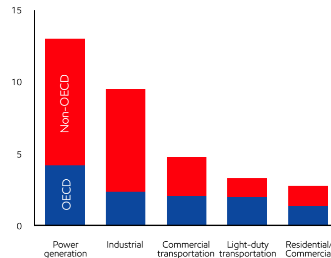
2017 global energy-related CO 2 emissions by sector
